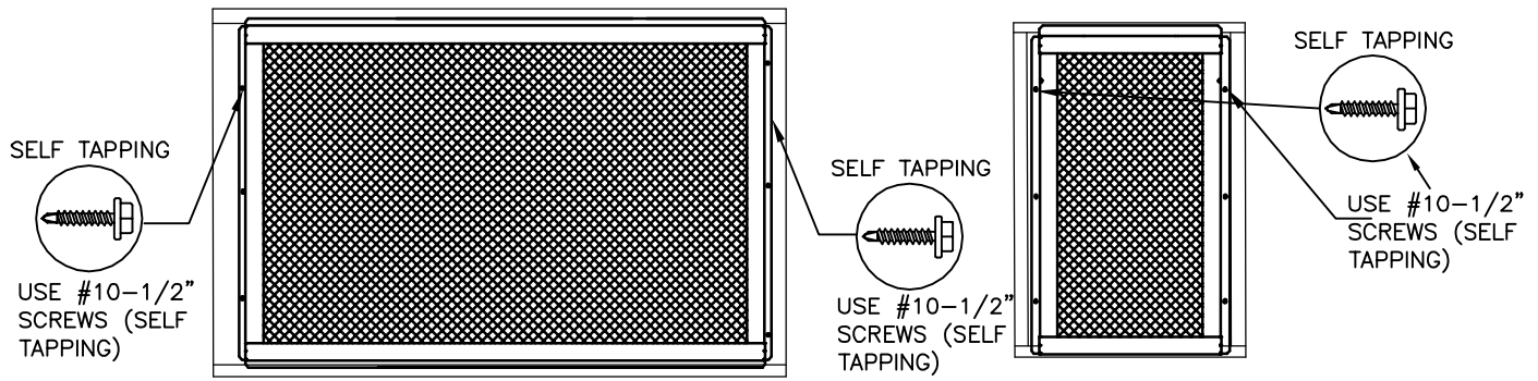
BACK VIEW
