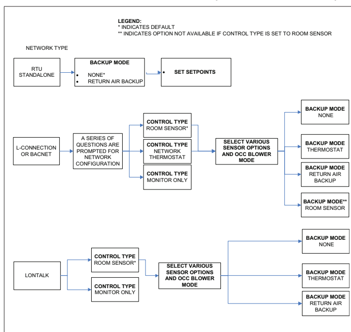
Figure 32. Backup Mode
