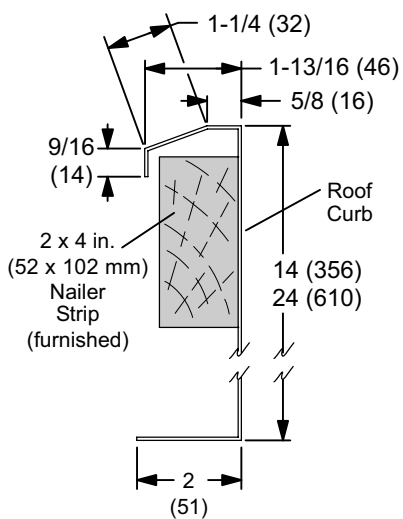
ROOF CURB SECTION A-A
