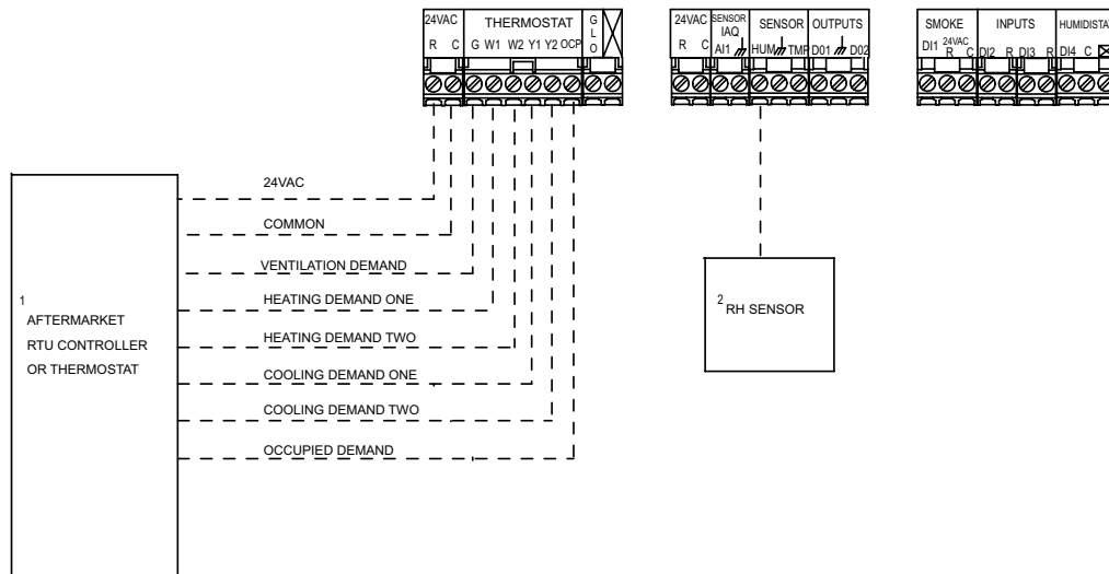
MSAV® (MULTI-STAGE AIR VOLUME) UNIT IN SINGLE ZONE APPLICATION
