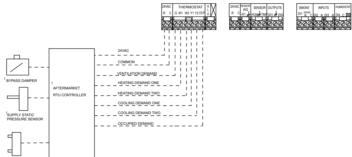
MSAV® (MULTI-STAGE AIR VOLUME) UNIT IN BYPASS ZONING APPLICATION
