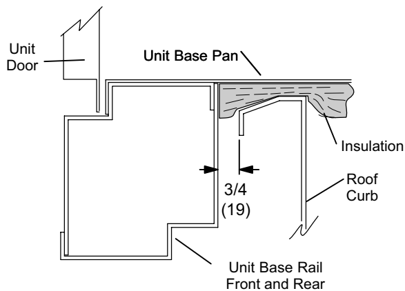
SIDE SECTION B-B With Unit Base Rail and Pan
