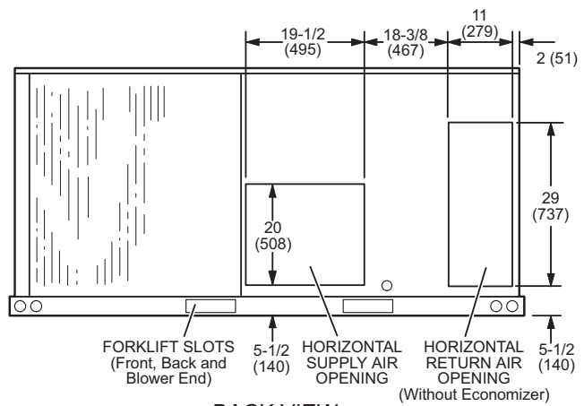
BACK VIEW
