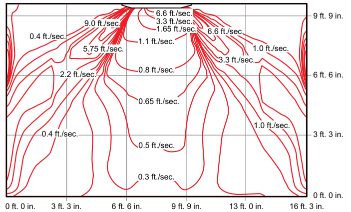
V33B036 - HEATING
