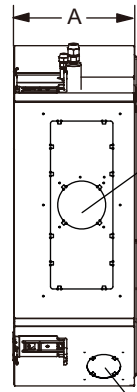
2-3/4 (70) dia. FRESH AIR INTAKE
