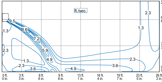
3MWMC036S4-1P - COOLING
